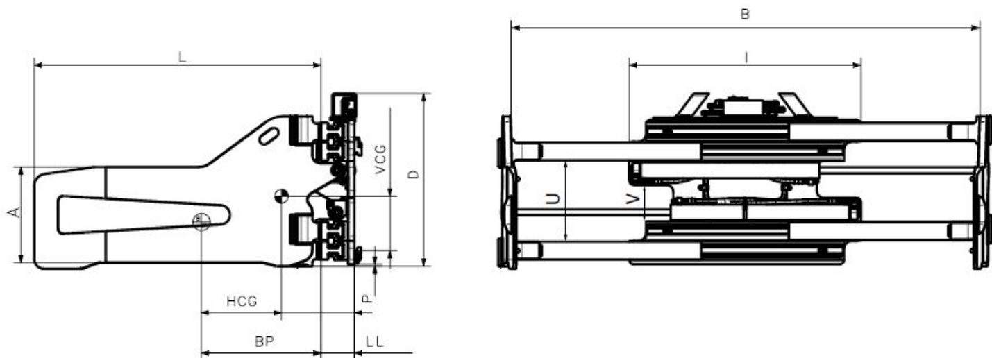
Model LC-G (with side shift)
